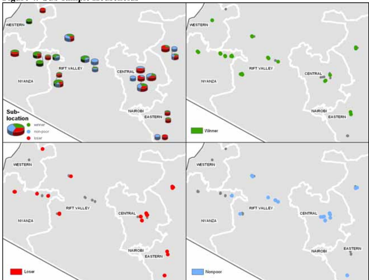
Figure 4. Sub-sample Households
